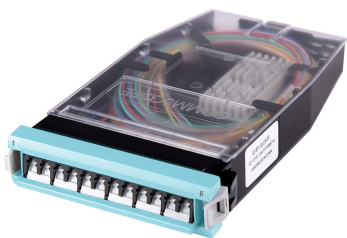
G2 Splice Cassette, 12LC with internal shutters, OM4, with pigtails
